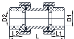
PP-R/PE-RT Change Union (Soc×Soc)
