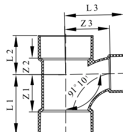
Large Radius Tee (D-LT)
