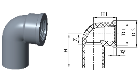
Faucet Elbow (AW)
