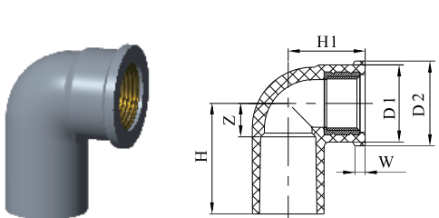
Faucet Elbow With Metal Insert (AW)
