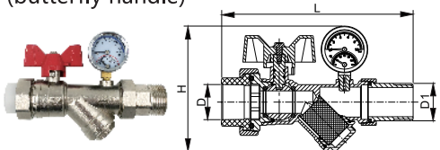
Long male thread ball valve with temperature gauge manometer (butterfly handle)
