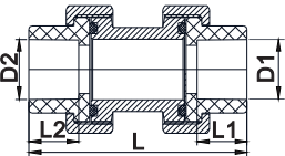
PP-R/PE Change Union (Soc×Soc)
