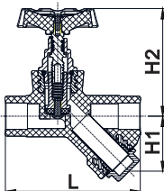
Y-style Stop Valve (Soc×Soc×Fipt)
