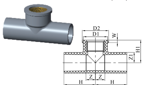
Faucet Tee With Metal Insert (AW)
