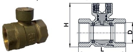
Lock Ball Valve (Fipt with Metal×Fipt with Metal)
