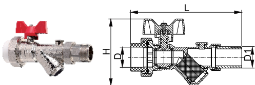
Long male thread ball valve with strainer (butterfly handle)
