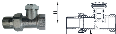
Straight Type Water Return Valve (Fipt with Metal×Mipt with Metal)
