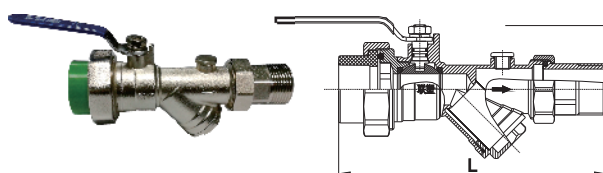
Nickel Plated Brass Ball Valve With Strainer 271 (Soc×Fipt with Metal)
