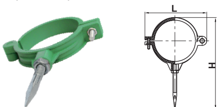
Pipe Clamp IV (Tusk Screw)
