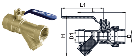
Brass Ball Valve With Strainer 261 (Soc×Fipt with Metal)
