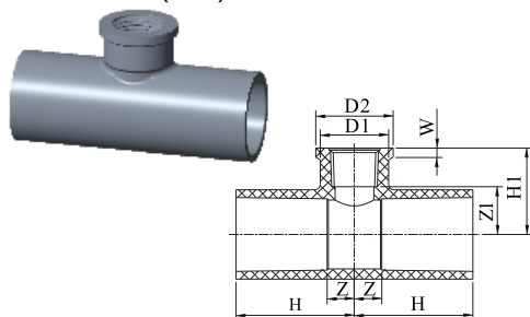
Faucet Tee (AW)
