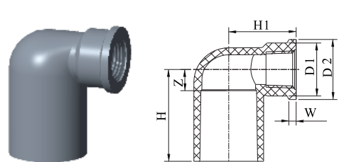
Faucet Elbow (AW)
