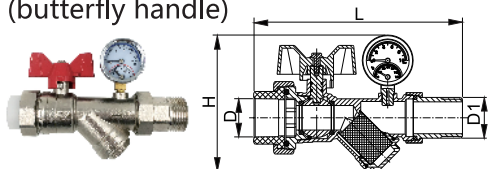
Long male thread ball valve with strainer meter (butterfly handle)
