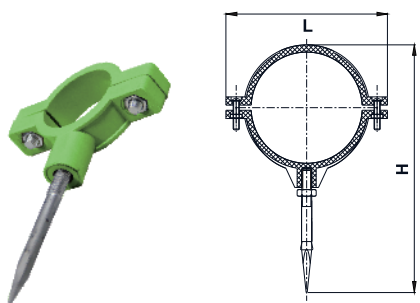
Pipe Clamp I (Tusk Screw)
