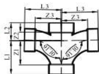
Large Radius Double Tee (D-WLT)
