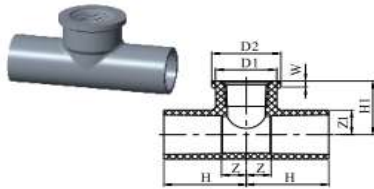
Faucet Tee With Metal Insert (AW)
