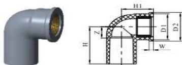
Faucet Elbow With Metal Insert (AW)
