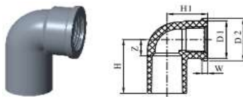
Faucet Elbow (AW)
