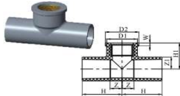
Faucet Tee With Metal Insert (AW)
